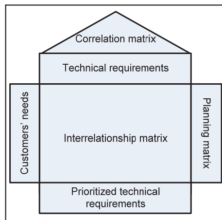
Fig. 1. HOQ matrix
