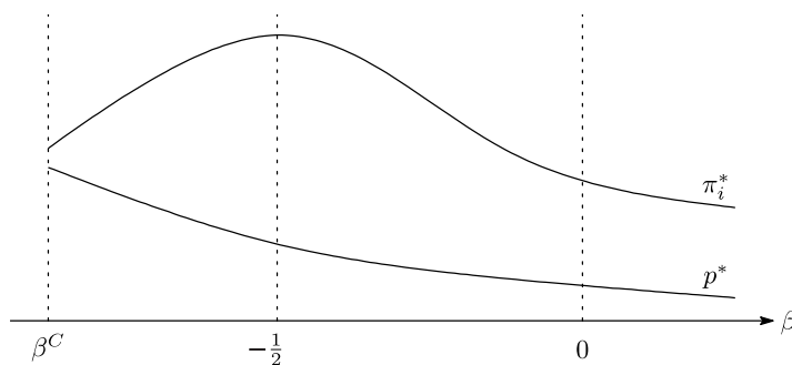
Fig. 1. Competition properties of equilibrium price and profits in the cartel region
