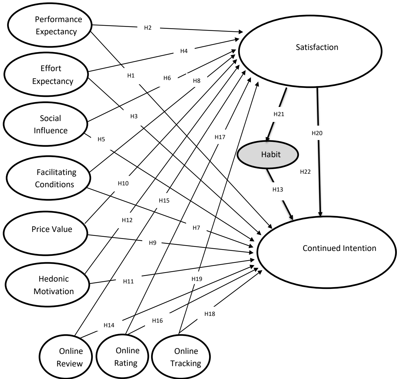
Fig. 1. Conceptual Framework
