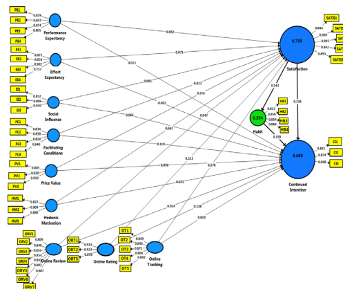
Fig. 2. Structural Model
