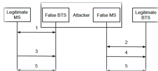
Fig. 5. MITM on GSM network via FBS method
