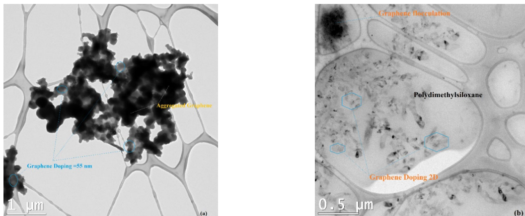
Fig. 7. TEM a) Graphene b) PDMS /Graphene solution
