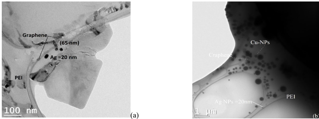
Fig. 8. TEM a) PEI –Graphene b) PEI-Graphene/NPs assembled.
