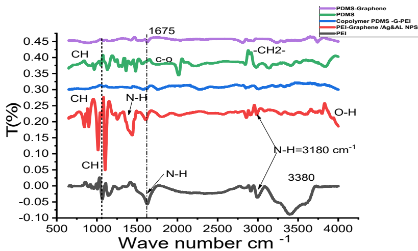
Fig. 3. IR spectrum characterization
