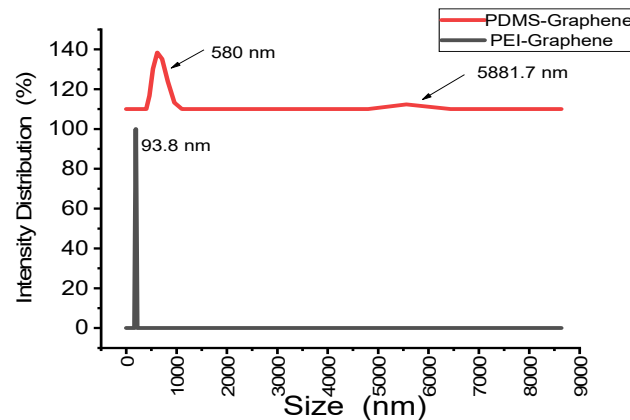
Fig.10. Particle size Analyzer a) PDMS /graphene b) PEI polymer assembled nanoparticles and graphene
