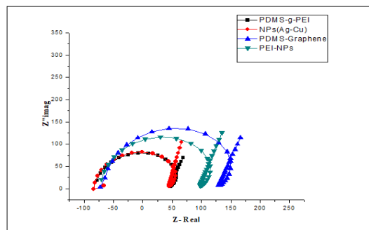
Fig. 2. The impedance of different prepared solutions used to copolymer composition.
