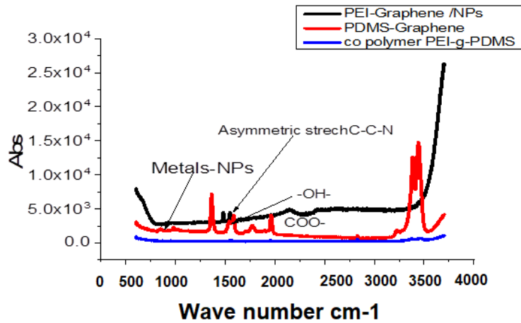
Fig. 4. Raman analysis for different composites.
