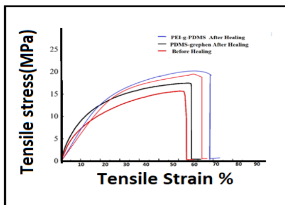
Fig. 13. Stress-strain of free-standing PDMS, and copolymers PDMS-graphene-PEI before and after the self-healing process
