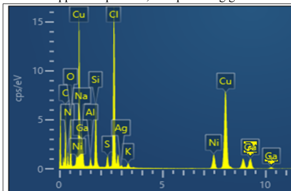
Fig. 11. EDAX characterization of copolymers
