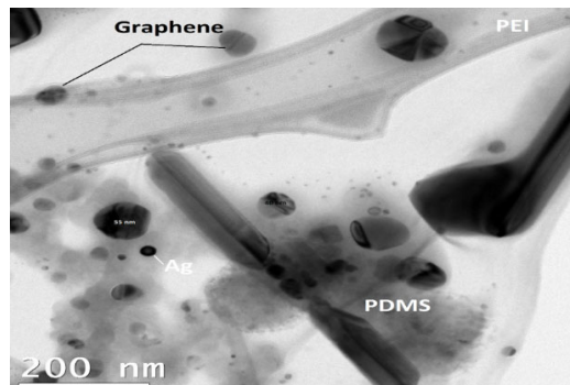
Fig. 9. TEM PDMS –Graphene /NPS –PEI Co-polymer composites.
